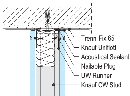
W111-VO1 Connection to ceiling
