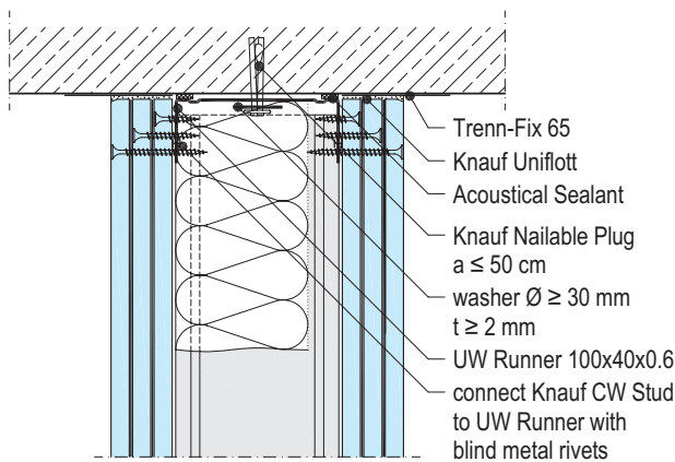
W118-VO1 Connection to ceiling
