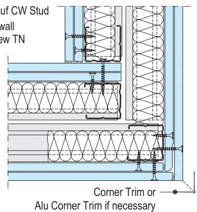
W115-D1 Corner
