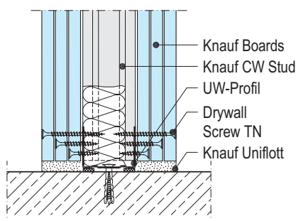
W113-VU1 Connection to floor
