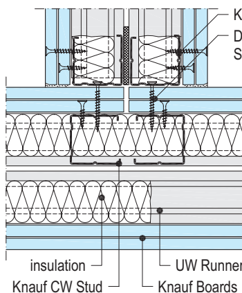
W115-C1 T-junction
