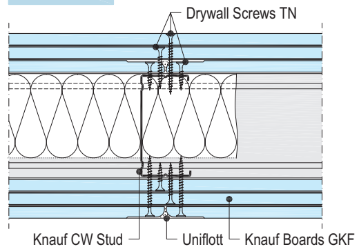
W118-B1 Joint
