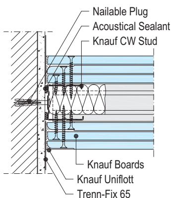
W113-A1 Connection to solid wall
