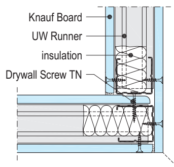
W111-D1 Corner
