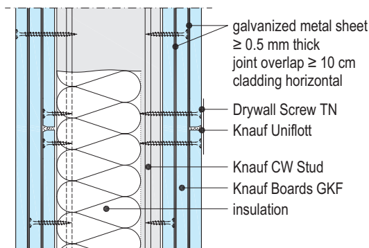
W118-VM1 Joint
