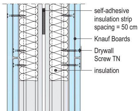
W115-VM1 Joint
