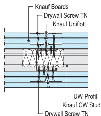
W113-B1 Joint
