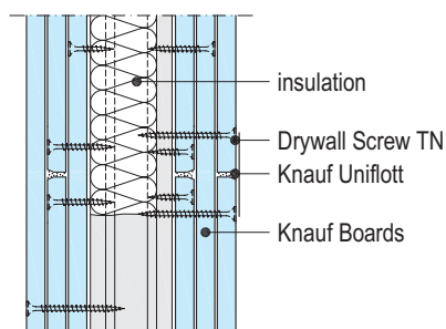
W113-VO1 Connection to ceiling
