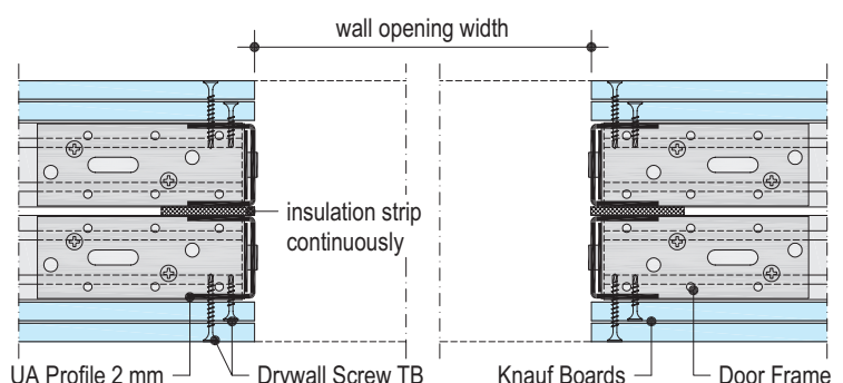
W115-E1 Door opening with UA Profile
