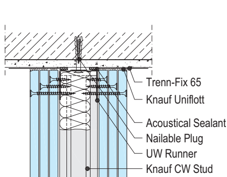
W113-VO1 Connection to ceiling
