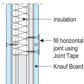
W111-VM1 Joint
