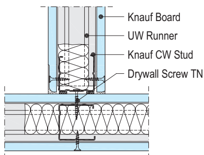
W111-C1 T-junction
