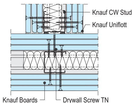
W113-A1 Connection to solid wall
