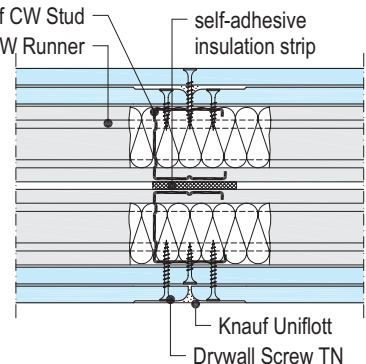
W115-B1 Joint
