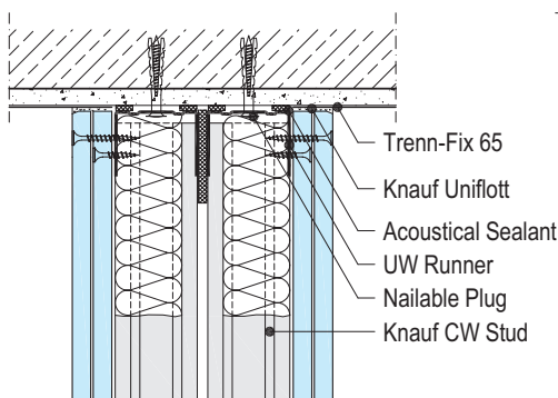
W115-V01 Connection to ceiling
