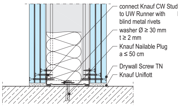
W118-VU1 Connection to floor
