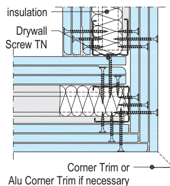
W113-D1 Corner
