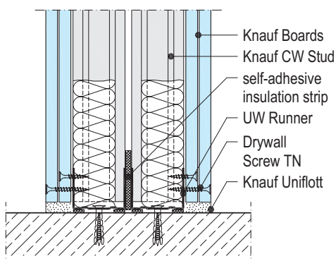
W115-VU1 Connection to floor
