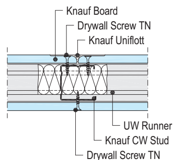
W111-B1 Joint
