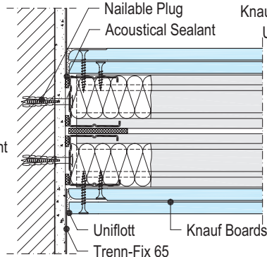
W115-A1 Connection to solid wall
