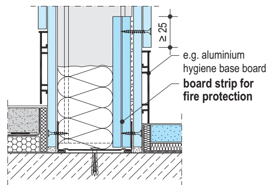
W112-VU3 Reduced connection to basic floor
