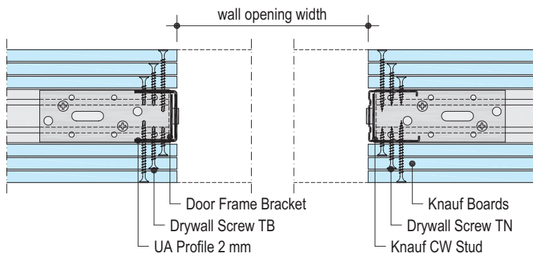
W113-E1 Door opening with UA Profile
